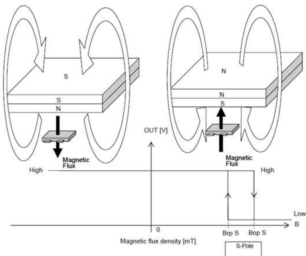
Fig 4, Magnetic Operation Characteristic of AS1810A
