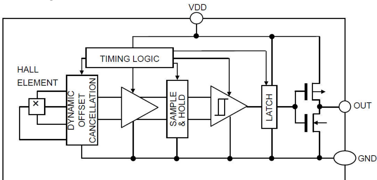
Figure 3, Block Diagram of AS1810A
